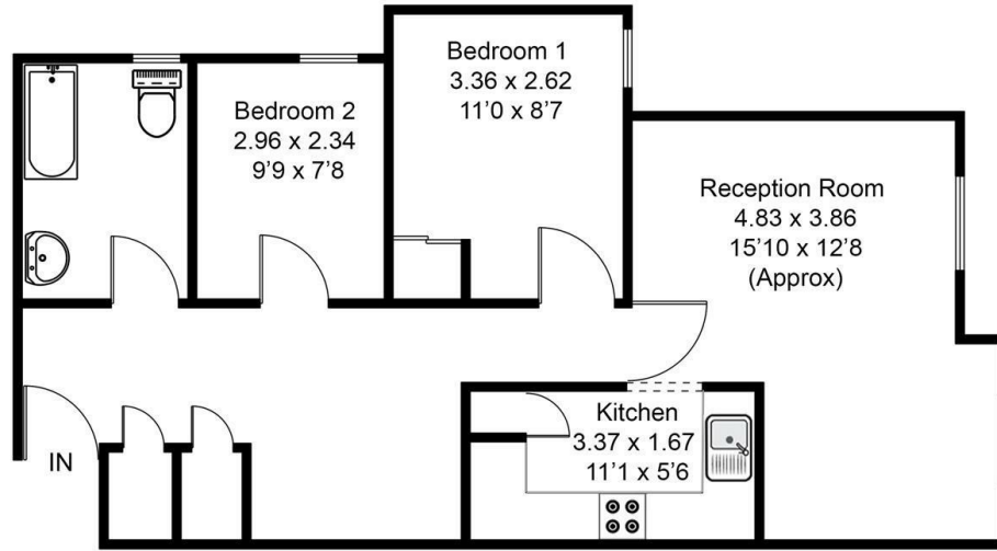
GROUND FLOOR FLAT
