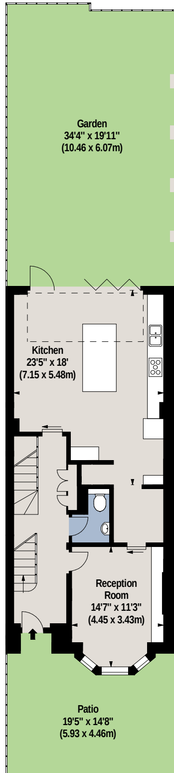
Ground Floor
