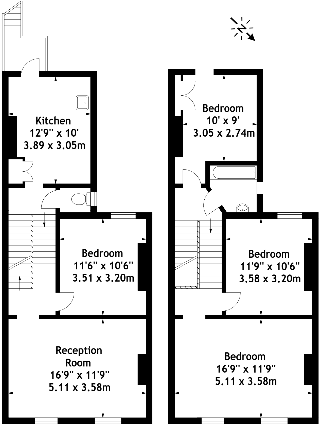
First Floor
