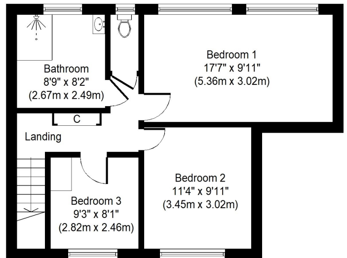
First Floor Approximate Floor Area 551 Sq. ft. (51.2 Sq. m.)
