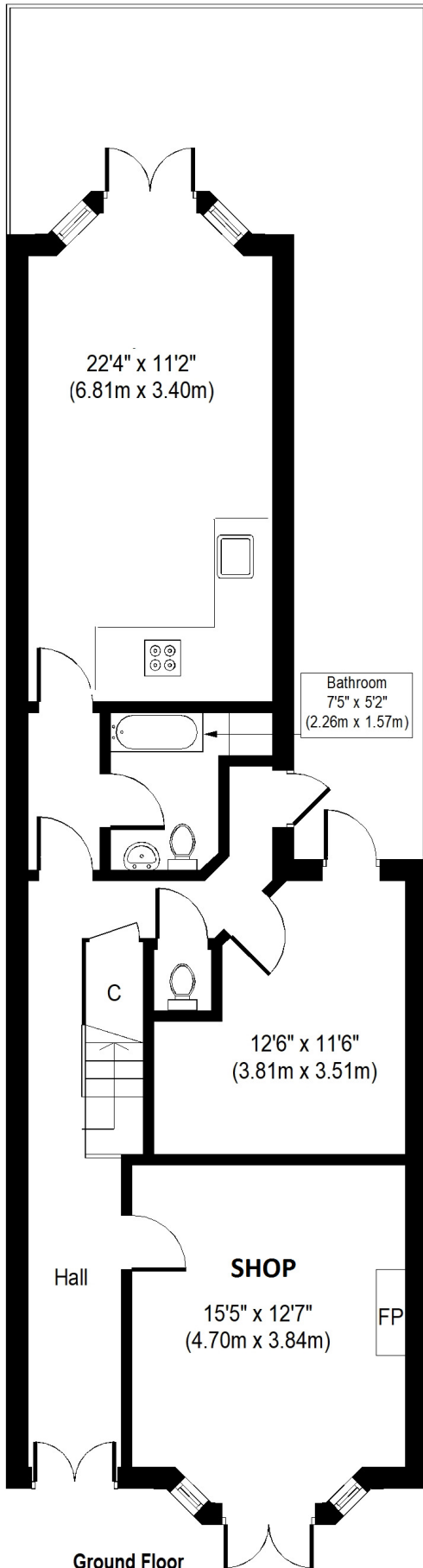
Ground Floor Approximate Floor Area 803 Sq. ft. (74.6 Sq. m.)
