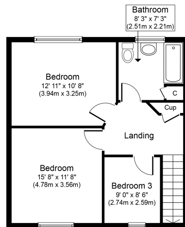
First Floor Approximate Floor Area 484 sq. ft. (45.0 sq. m.)
