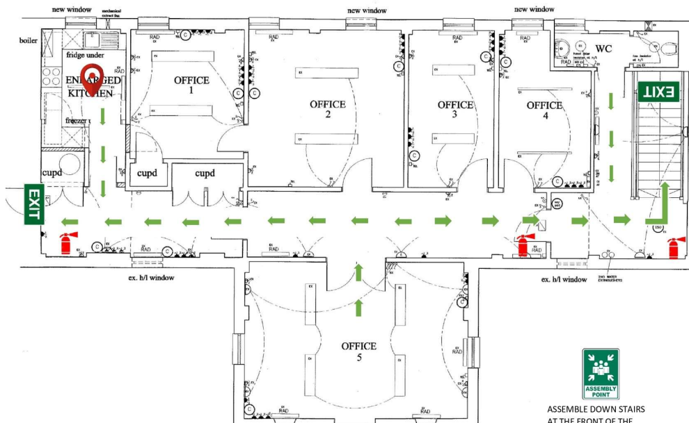
First Floor Plan – for identification purposes only
