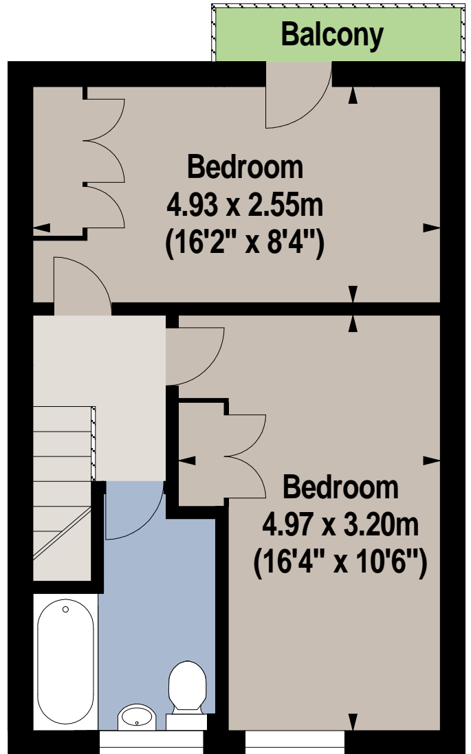
Third Floor
