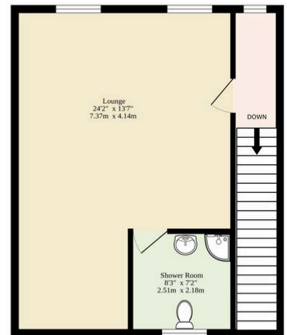
2nd Floor 426 sq.ft. (39.6 sq.m.) approx.
