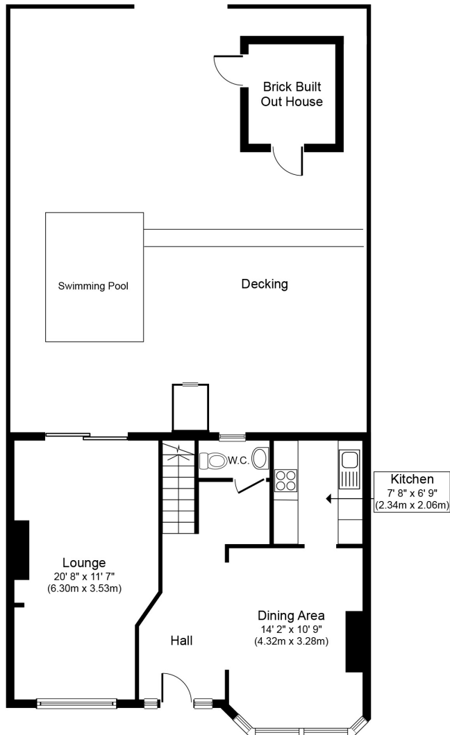
Ground Floor Approximate Floor Area 667 sq. ft. (62.0 sq. m.)
