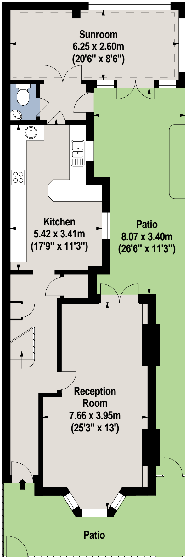
Ground Floor
