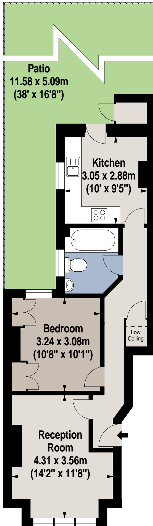
Ground Floor
