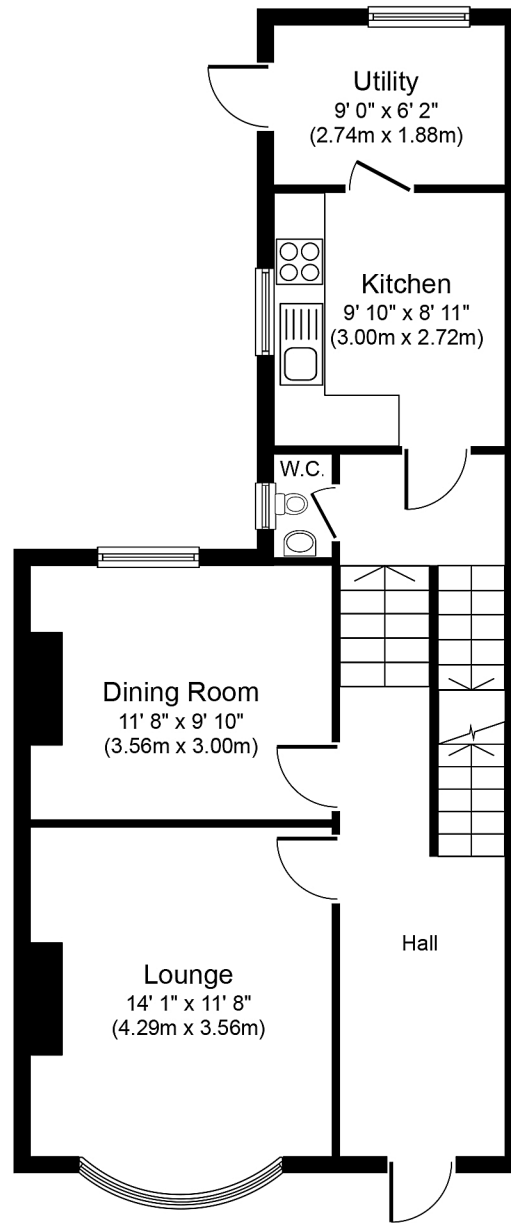
Ground Floor Approximate Floor Area 618 sq. ft. (57.4 sq. m.)
