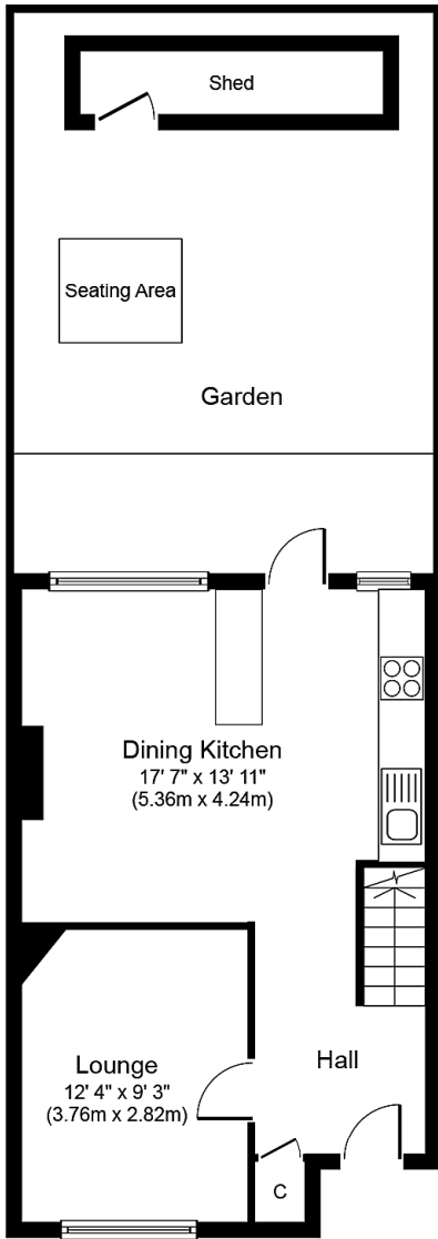
Ground Floor Approximate Floor Area 439 sq. ft. (40.8 sq. m.)
