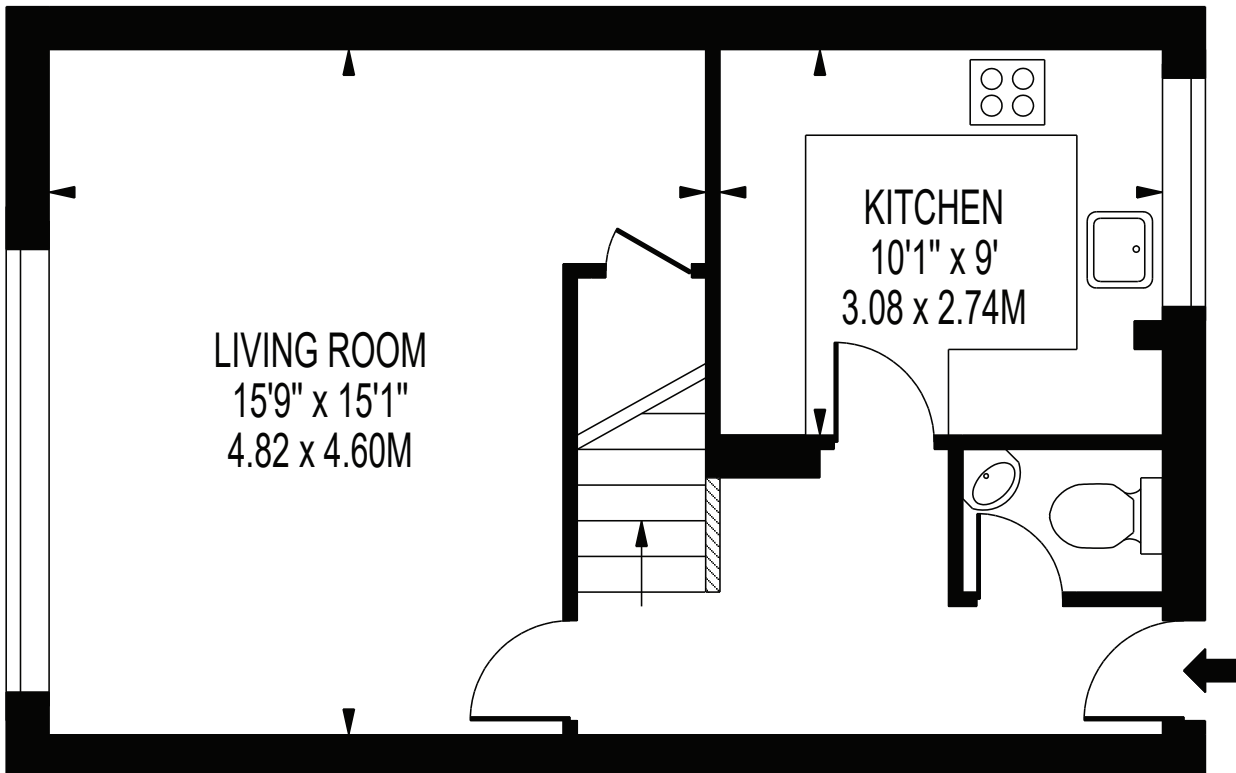
SECOND FLOOR
