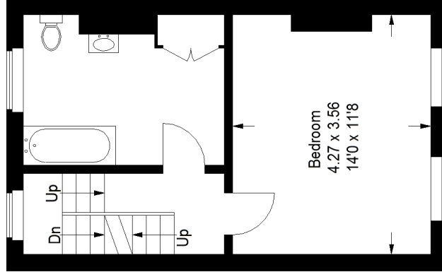
Second Floor
