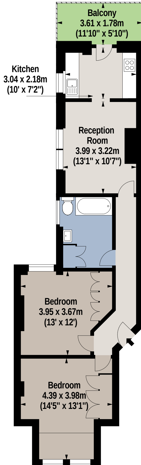
First Floor
