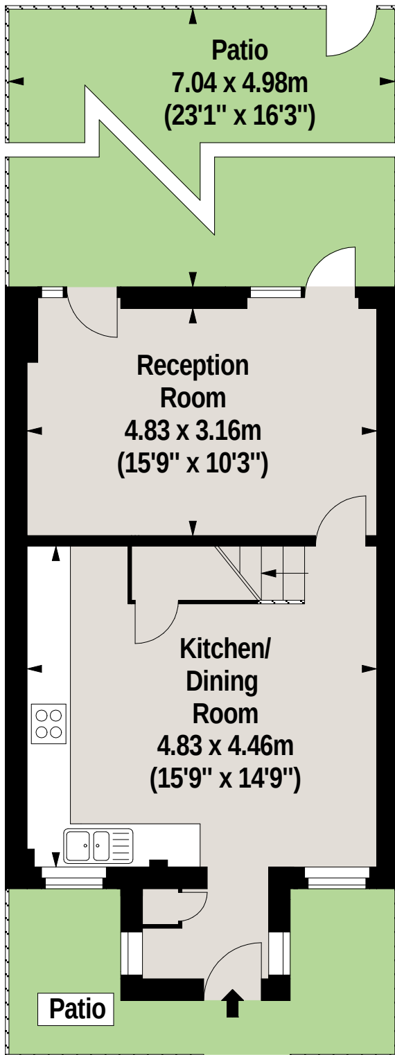
Ground Floor
