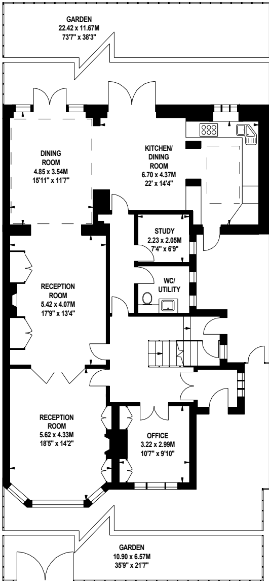
Ground Floor 1526 sq ft
