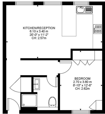
Third Floor 438 ft 2
