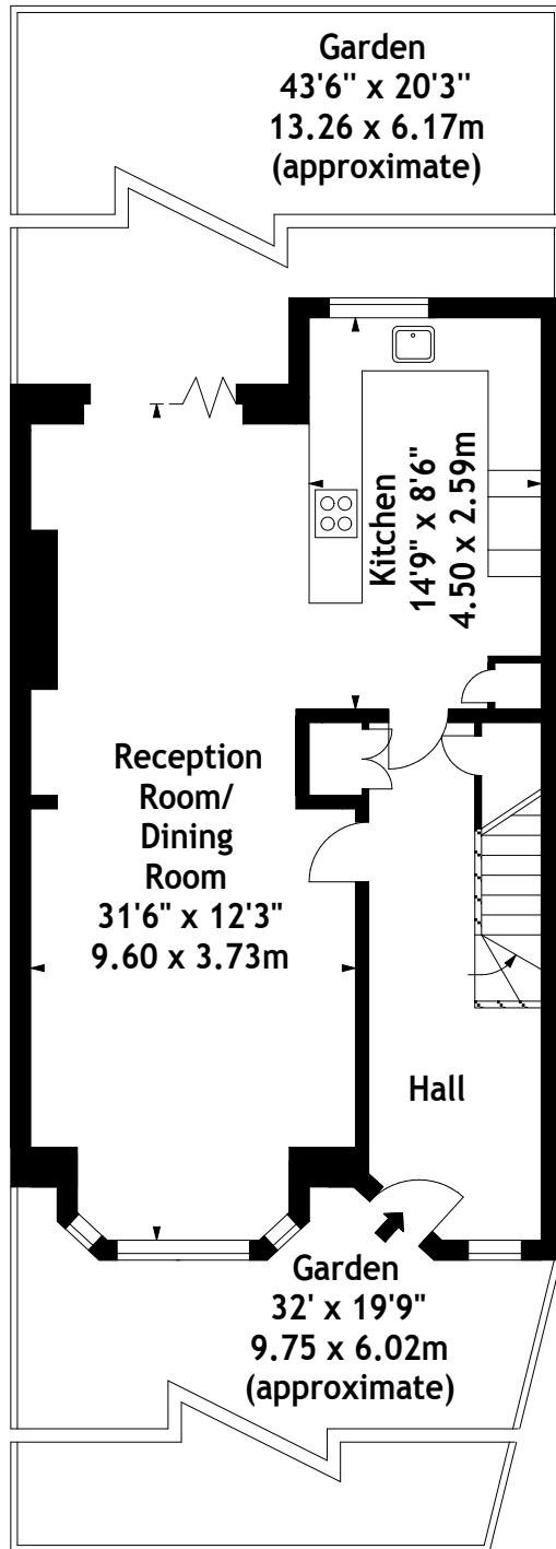
Ground Floor
