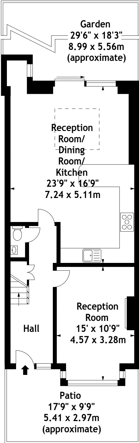
Ground Floor
